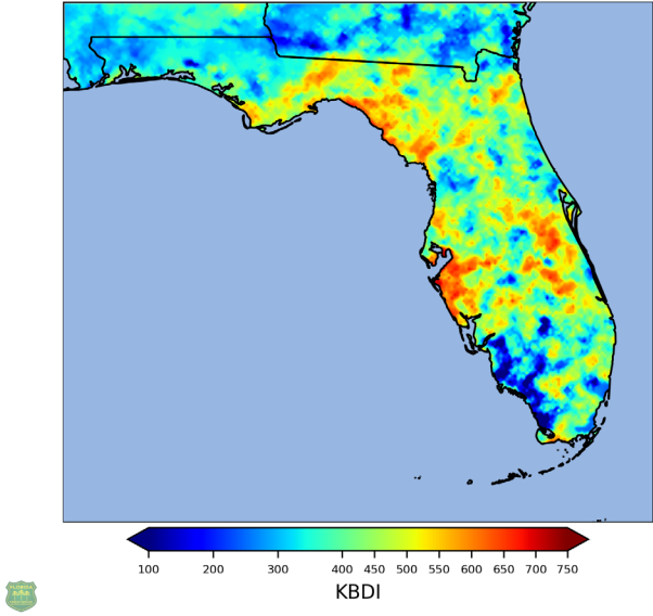
Keetch-Byram Drought Index | Mon 06/15/26, 02:00 PM EDT
