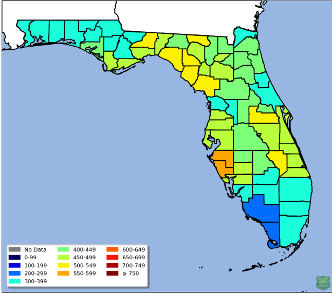
KBDI Averages by County | Mon 06/15/26
