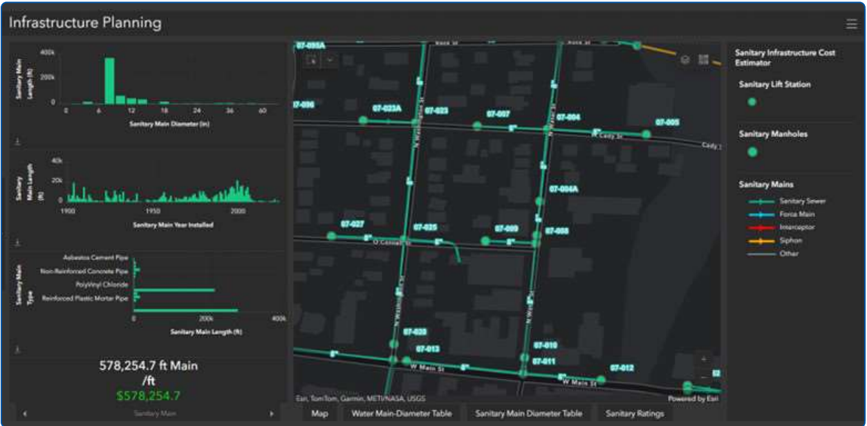
SAMPLE DASHBOARD 2
